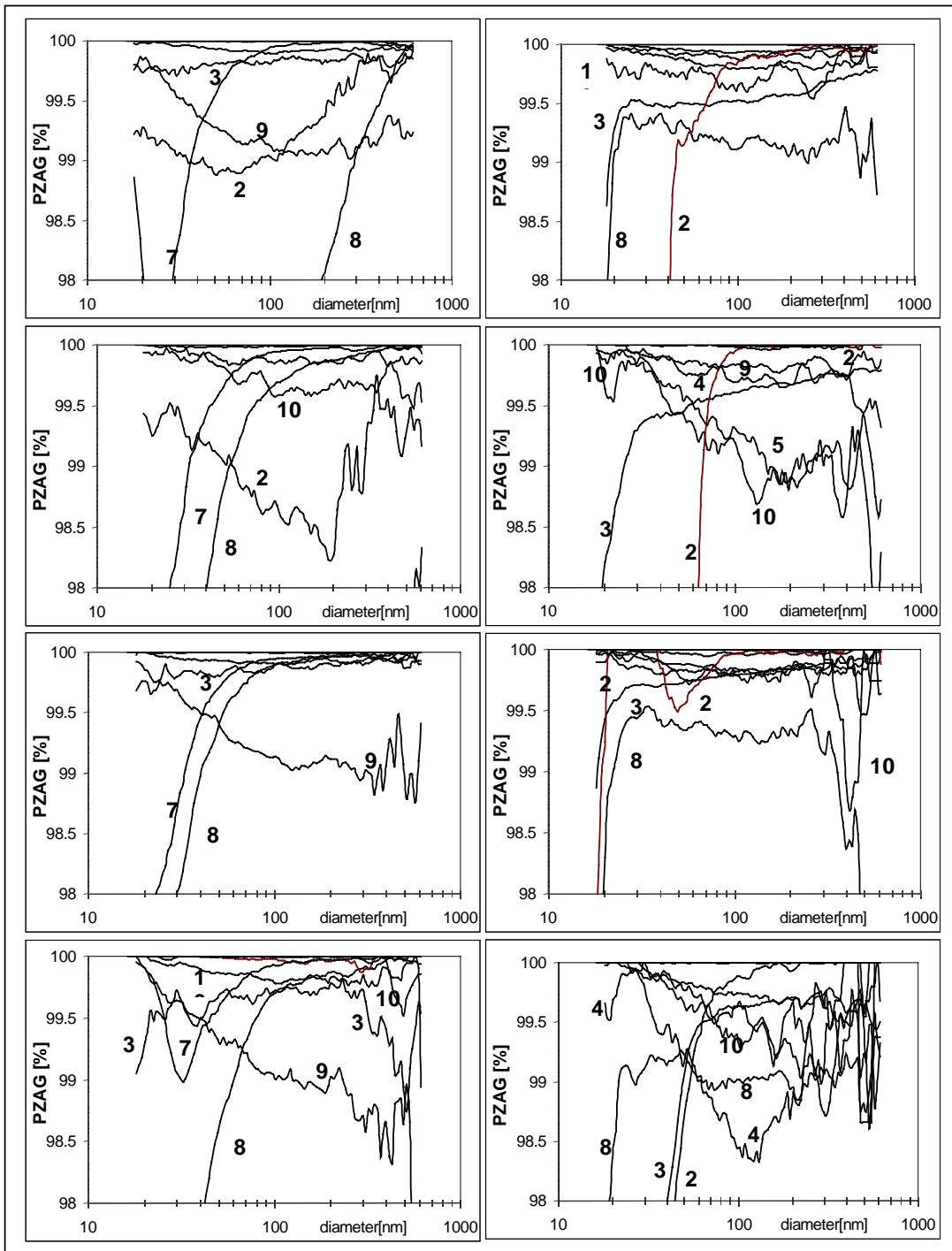
Fig.4: Filtration efficiency based on number count PZAG for 10 VERT-approved particle filter systems Left: VFT1, the new filter. Right: VFT3, the same filter after > 2000 operation hours in a typical application. Top to bottom: ISO 8178, 4 operation points: nominal rpm/full-load - nominal rpm/50%-part-load - part rpm /full-load and part rpm/part-load. Some data is >99,9 % efficiency, so close to the boundary that they cannot be distinguished and are not charted
