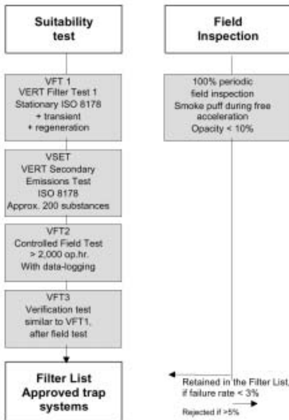
Fig.2: Overview of VERT suitability test [13]
