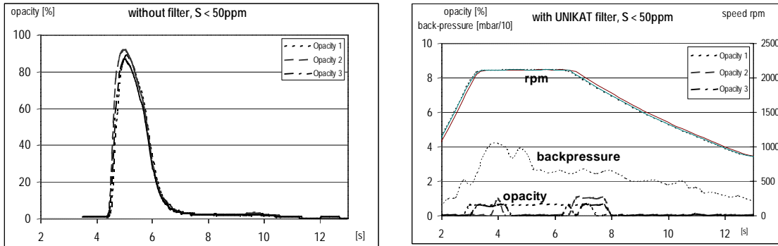
Fig.3: Opacity during free acceleration with/without particle trap.
